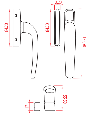
Cremone with Latch System Mandallı Kol
